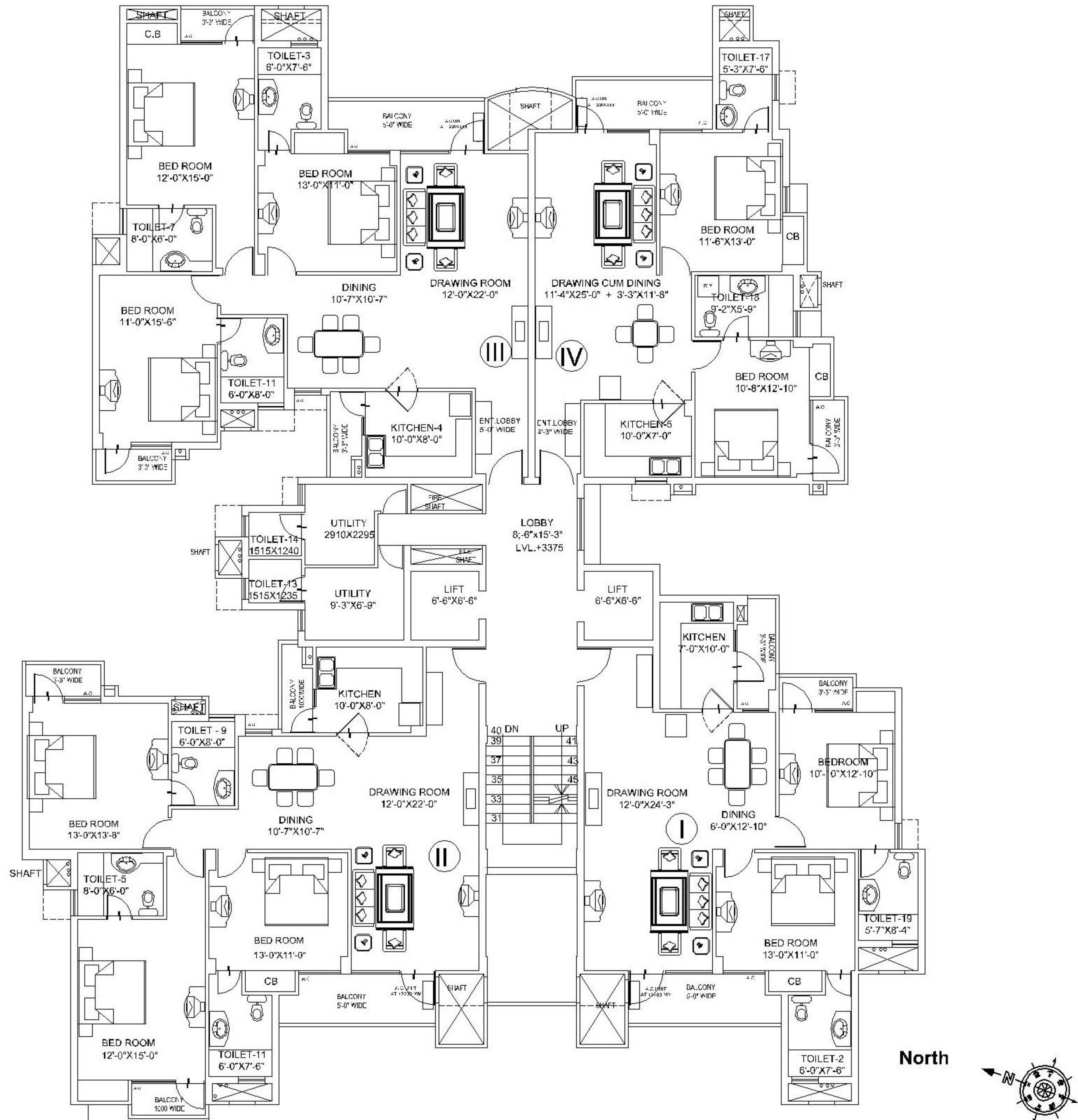
TYPICAL FLOOR PLAN CLUSTER PLAN ( TOWER - L ) ( G + 6 )
